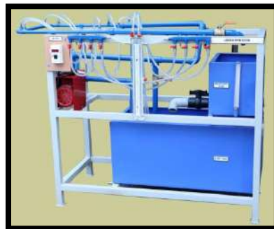
LOSSES IN PIPE FITTING
