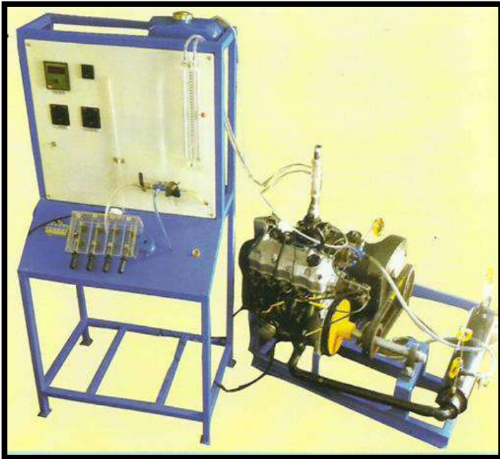
MULTI CYLINDER PETROL ENGINE TEST RIG WITH ELECTRICAL LOADING
