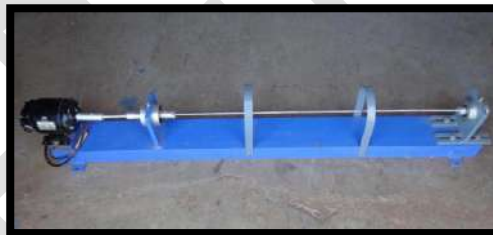
WHIRLING OF SHAFT APPARATUS
