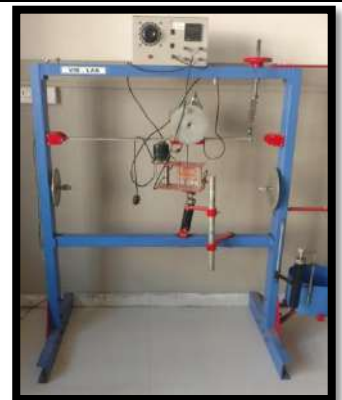
FORCED VIBRATION SET UP
