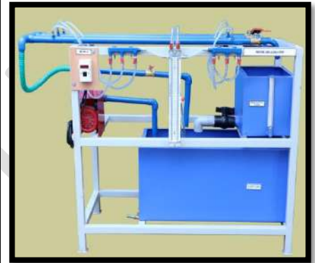
PIPE FRICTION APPARATUS
