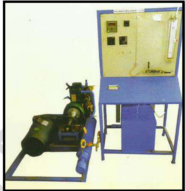
SINGLE CYLINDER DIESEL ENGINE TEST RIG WITH ELECTRICAL LOADING
