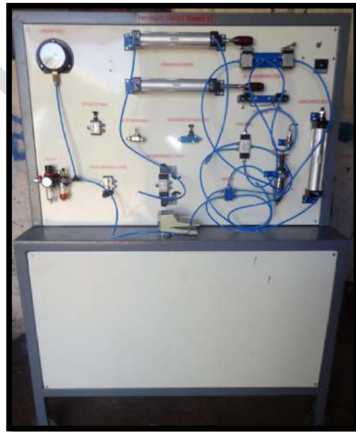
BASIC PNEUMATIC CIRCUIT TRAINER KIT
