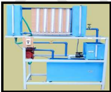
BERNOULLI'S THEOREM
