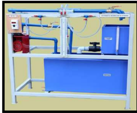
VENTURI AND ORIFICE METER APPARATUS
